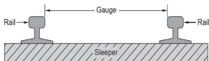
Gauge
