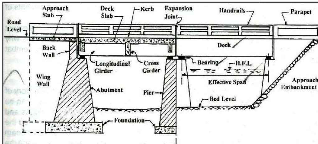
Figure 1 Components of a Typical Bridge.
